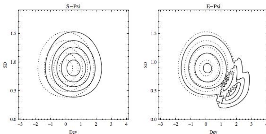
FIGURE 8. S & E-PSI VIA t(5) -(TRIAL JUB FN)
