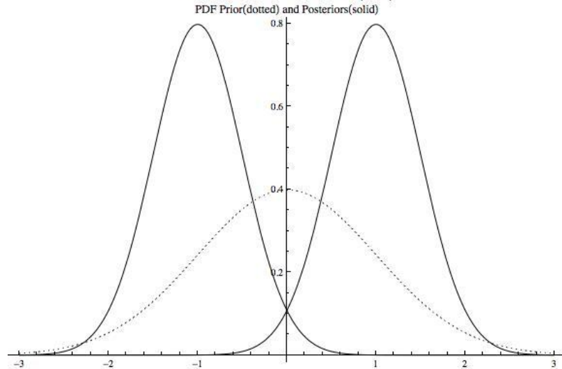
FIGURE 5. E-PSI VIA t(\text{diff})
