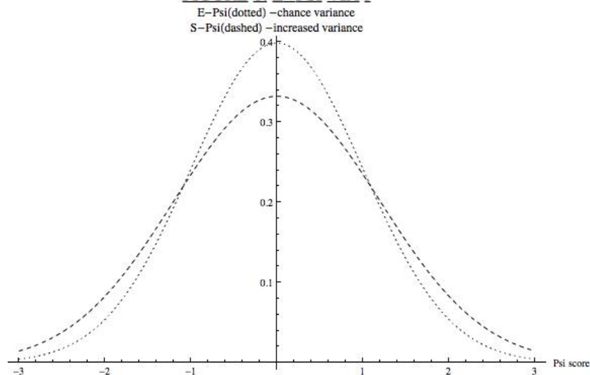
FIGURE 6. E-PSI VIA r
