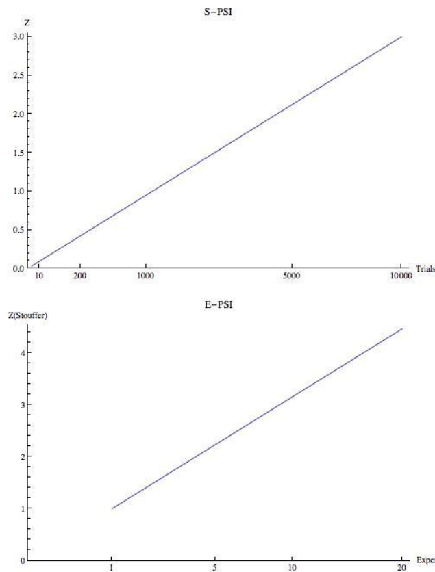
FIGURE 3. GROWTH OF Z WITH (RELEVANT) N FOR S-PSI and E-Psi x scaled as Sqrt[n]
