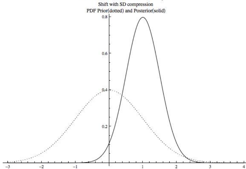
FIGURE 4. E-PSI VIA t/F
